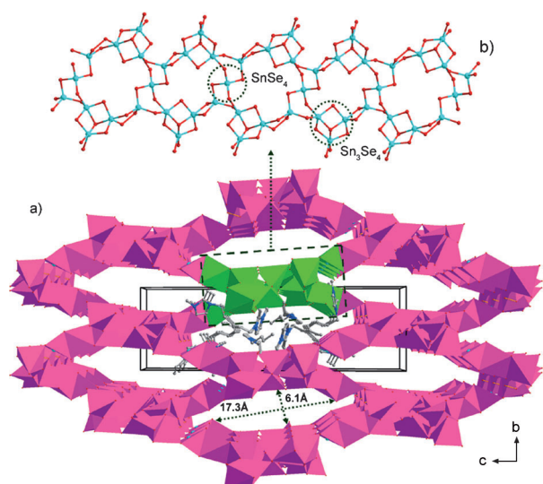
Figure 2. a) Polyhedral view of the structure of 2 along the a -axis. Most of the [\text{bmmim}]^+ (blue/gray stick models) in channels are omitted for clarity. b) View of the [\text{Sn}_9\text{Se}_{17}(\text{Se}_2)_{0.9}\text{Se}_{0.1}] double-chain in 2 (highlighted in green in (a)) extended along the a -axis. The disordered (\text{Se}_2)_{0.9}\text{Se}_{0.1} units are drawn as (\text{Se}_2) for clarity.
